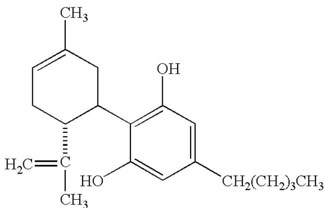
Cannabidiol (CBD)
